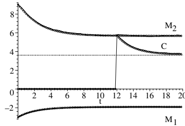
Fig. 5.13. As in Fig. 5.12 but for t' = 12 . As shown by the first and second moments in this case we are in the stationary regime. The thin horizontal line describes M_{1,\text{st}}^2 ; reprinted from [182], © 2004, with permission from Elsevier
