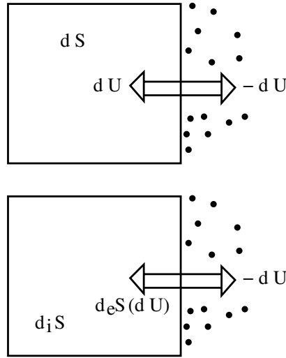
Fig. 4.2. Two kinds of entropy changes: d_i S and d_e S . The environment is considered as an ensemble of heat bath particles (which are represented by full dots)
